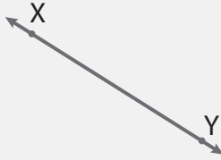
Line \overleftrightarrow{XY}
