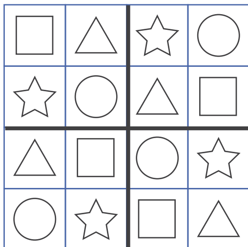
4 by 4 Shape Sudoku
